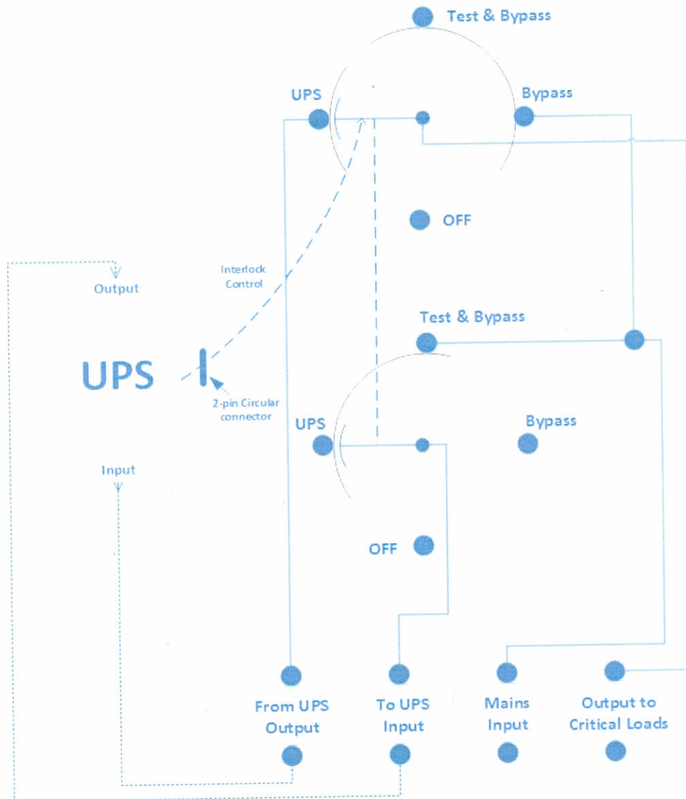
External Maintenance Bypass Switch Hardwired
